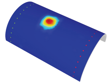
The tomography software shows the location and depth of any corrosion or erosion
