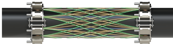
Illustration of signal paths with 16 transducers on a horizontal pipe, giving 100% coverage with multiple redundancy signal paths
