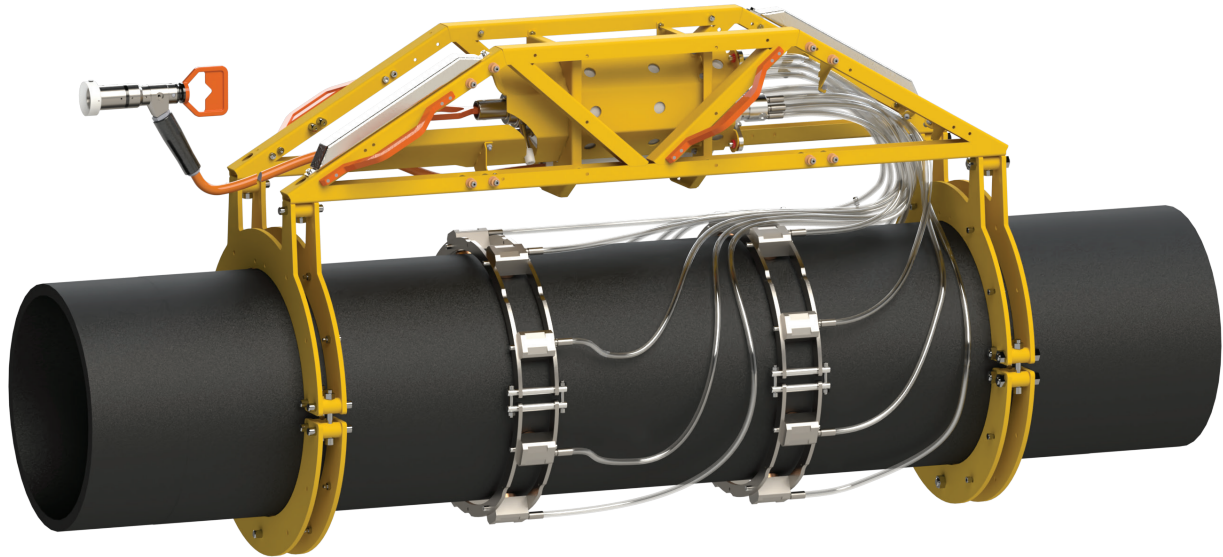
ClampOn Subsea CEM® Corrosion-Erosion Monitor
